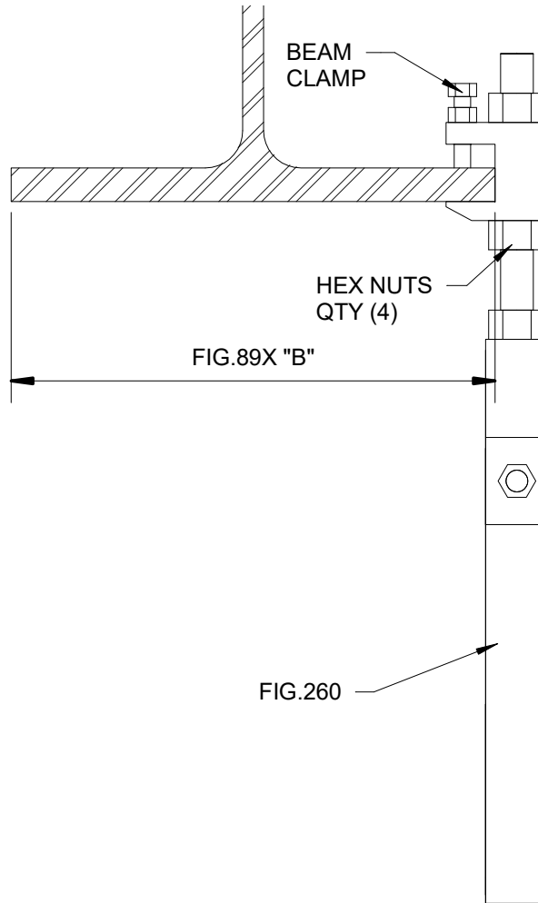
SIDE VIEW
